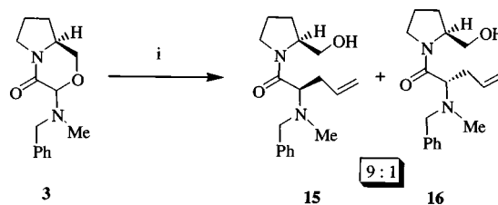
Scheme 6. \text{TiCl}_4 -mediated allylation of 3 : i) \text{TiCl}_4 , allyltrimethylsilane, dichloromethane, -78^{\circ}\text{C} , 4 h
