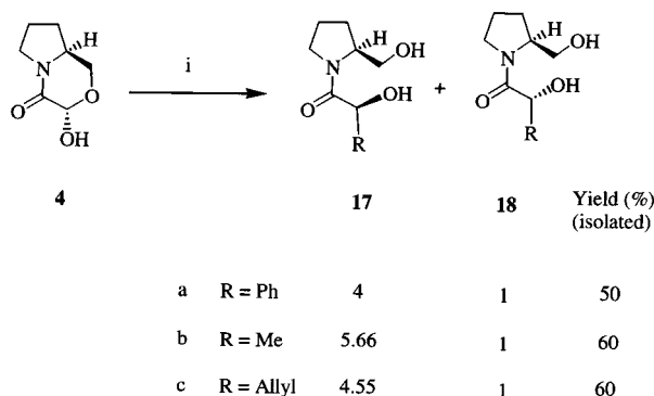
Scheme 7. Stereoselective alkylation of 4 using Grignard reagents: i) RMgX, THF, –40°C, room temperature, 6 h
