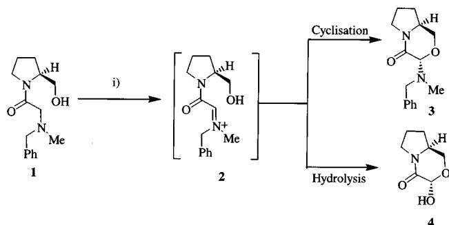
Scheme 1. PET activation of 1-( N -benzyl- N -methylglycyl)-( S )-prolinol ( 1 ): i) hv, DCN/MV ++ , CH 3 CN
