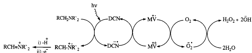
Figure 1. A photosystem to effect sequential two-electron oxidation of amines
