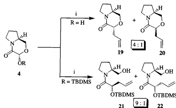
Scheme 8. TiCl 4 -mediated allylation of 4 : i) TiCl 4 , allyltrimethylsilane, dichloromethane, –78°C, 4 h
