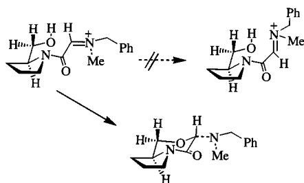
Figure 2. Transition-state model to explain the stereoselectivity during the PET cyclisation of 1
