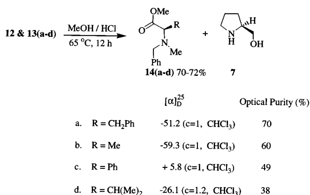
Scheme 5. Hydrolysis of substrates 12 and 13
