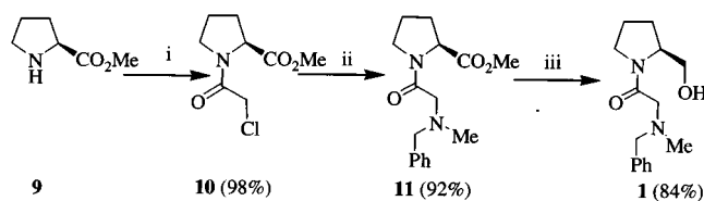
Scheme 3. Synthesis of 1-( N -benzyl- N -methylglycyl)-( S )-prolinol ( 1 ): i) ClCH 2 COCl, NaHCO 3 /H 2 O, 2 h; ii) PhCH 2 (Me)NH, K 2 CO 3 /CH 3 CN, 6 h; iii) NaBH 4 , EtOH, 12 h
