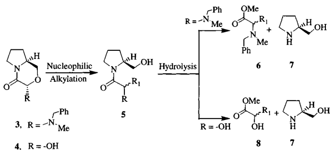
Scheme 2. Proposed stereoselective alkylations of substrates 3 and 4
